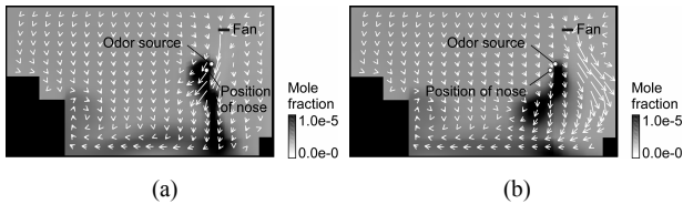
Fig. 3. Results of CFD simulation for the scenario assumed in the sensory tests. Top view of the odor distribution and airflow field in the horizontal cross section at 0.1 m from the floor are presented. (a) and (b) are the snapshots of the odor distribution and airflow field at 288 s and 293 s, respectively. The velocity vectors shown in the figures are in the range of 0 to 0.75 m/s.
