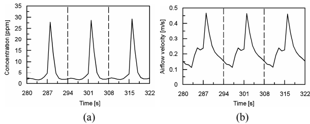
Fig. 4. Time courses of (a) the odor concentration and (b) the airflow velocity at the assumed position of the panelist's nose after 20 cycles of oscillation of the fan. The values were extracted from the CFD simulation data. Periodic changes in the odor concentration and the airflow velocity were observed.
